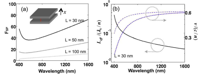
FIG. 3. (Color online) (a) Emission enhancement factor for a MDM slab (due to the gap SPP excitation) as a function of \lambda_0 . (b) Normalized group velocity (dashed line), phase velocity (dashed-dotted line), and mode length (solid line) for L=30 nm.
